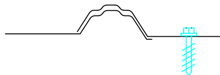
Multi-rib edge lap
