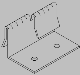
Panel Clip
